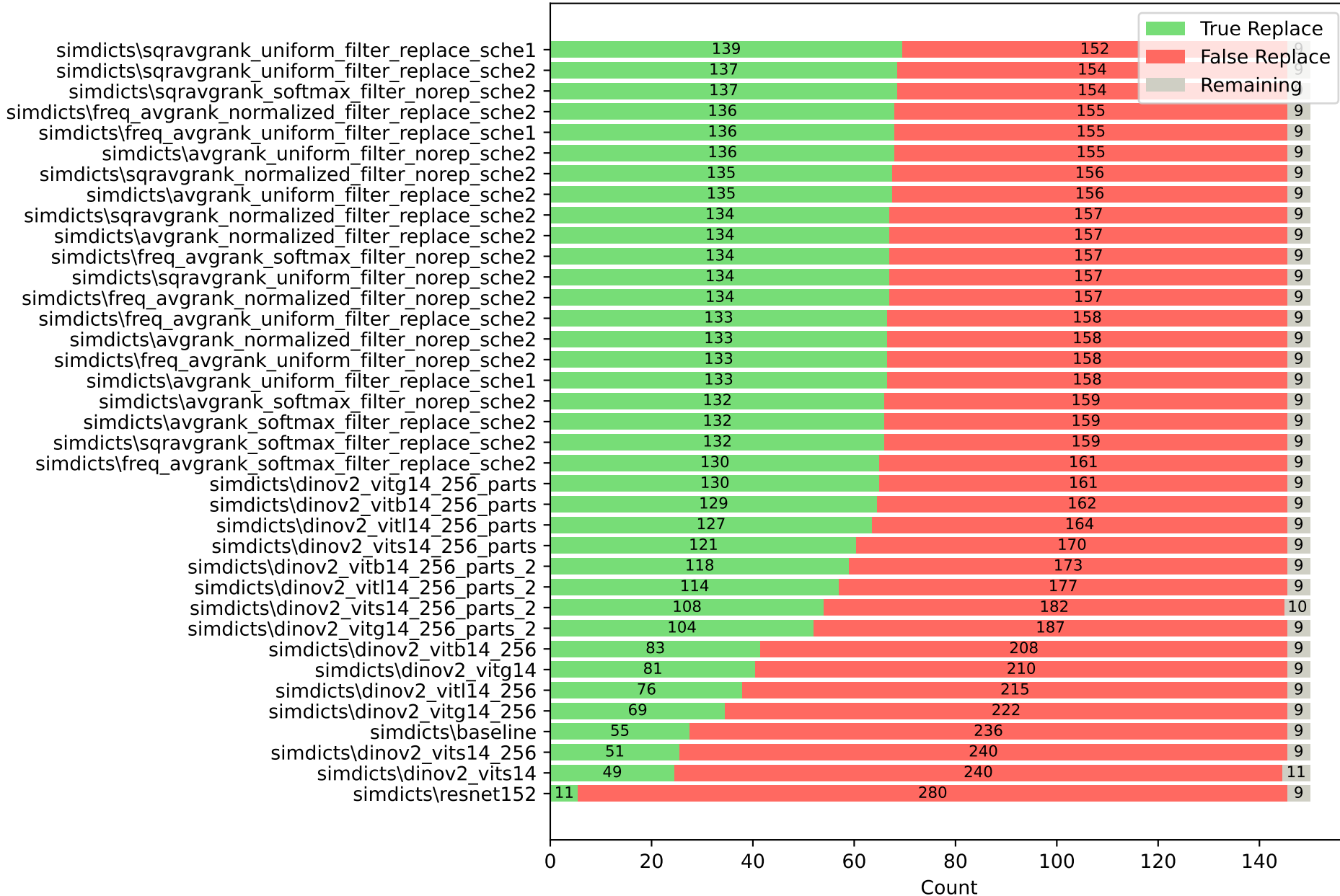
Similarity Dictionary Performance
